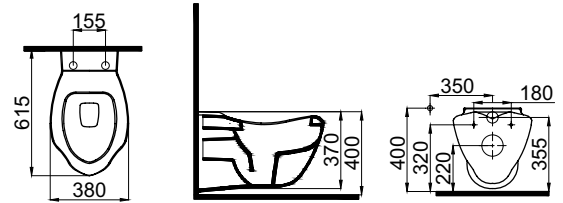
6104-0605 Mialuce Manta Asma Klozet (38x61x37) Wall Hung WC Pan
