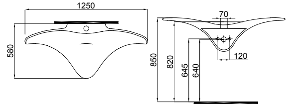
6101-1255 Mialuce Manta Monoblok Lavabo (58x125) Monoblock Washbasin
